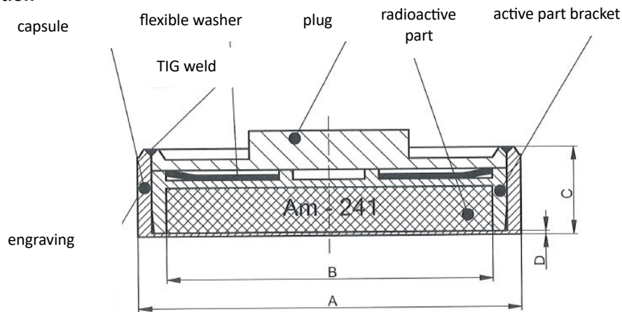
Figure 1: SFRM of the construction type Am1.GXX. The illustration corresponds to the technical drawing “Am1.GXX ASSEMBLY, drawing No. 2001, Eckert & Ziegler Cesio Ltd., 25 August 2020.” The dimensions of the individual subtypes are given below in the SFRM Parameters section.
