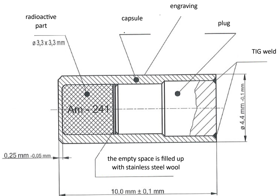
Figure 1: SFRM of the construction type Am1.P08. The illustration corresponds to the technical drawing "Am-241 source Am1.P08, 1.207.01.08-00:00(4), Eckert & Ziegler CESIO" of 25 August 2020.
