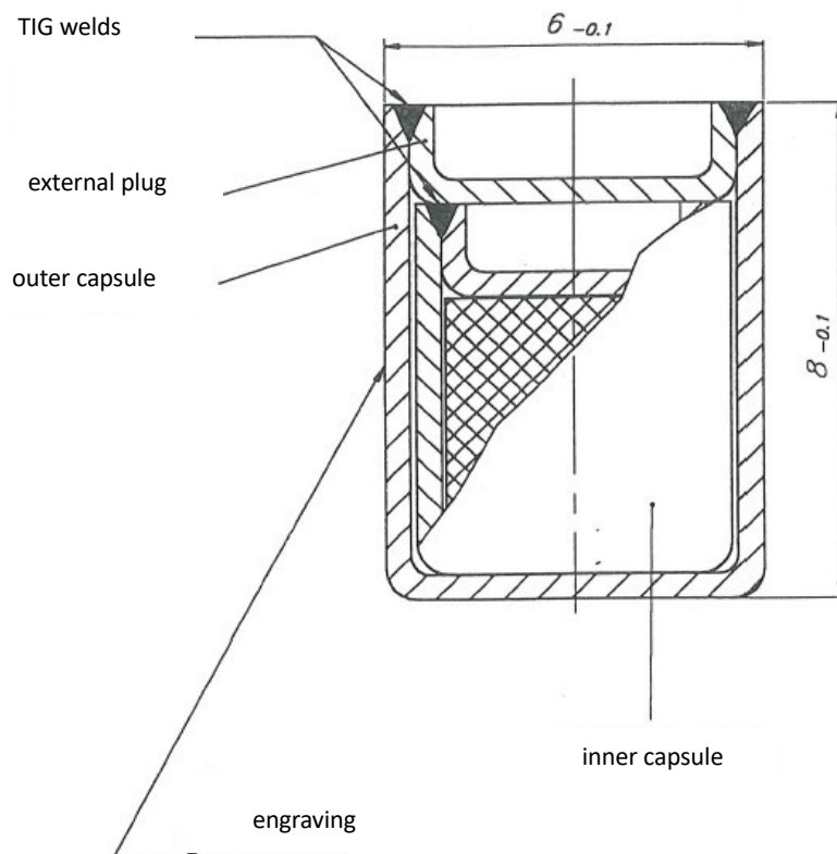
Figure 1: The SFRM of the construction type Cs7.P03. The illustration corresponds to the technical drawing "Cs-137 Quelle Cs7.P03, 1.203.03.03-00:00(4), BEBIG Isotopentechnik und Umweltdiagnostik GmbH" of 9 November 1995.
