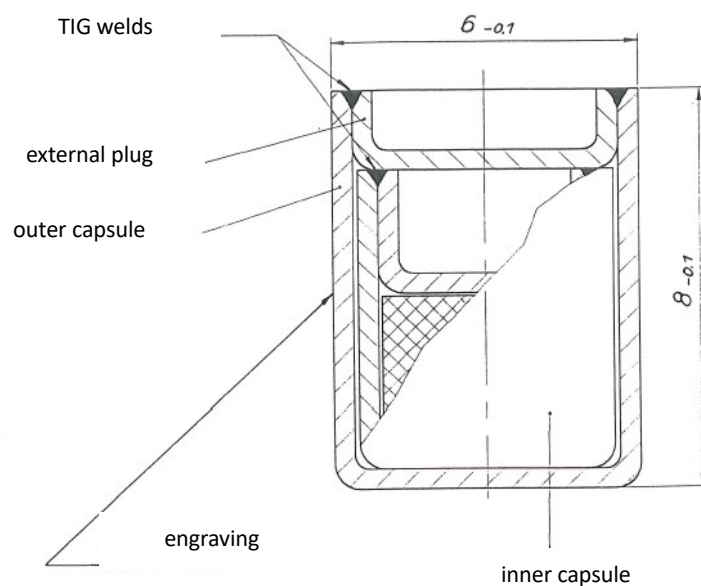
Figure 2: SFRM of the construction type Cs7.P10. The illustration corresponds to the technical drawing “Cs-137 Quelle Cs7.P10, 1.203.03.07-00:00(4), BEBIG Isotopentechnik und Umweltdiagnostik GmbH” of 22 May 1995.
