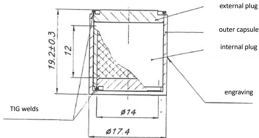
Figure 1: SFRM of the construction type Am1.N09. The illustration corresponds to the technical drawing "Am-Be Neutronenquelle Am1.N09, 1.207.02.05-00:00(4), BEBIG Isotopentechnik und Umweltdiagnostik GmbH, Berlin", 16 July 1995.
