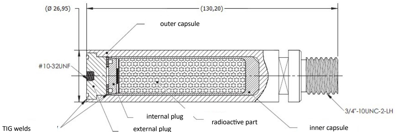
Figure 1: SFRM of the construction type Am1.N03. The illustration corresponds to the technical drawing "MODEL BP SERIES, CAPSULE 4103 (Am1.N03), drawing No. BP-REG, Eckert & Ziegler Isotope Products, Valencia, California 91355".
